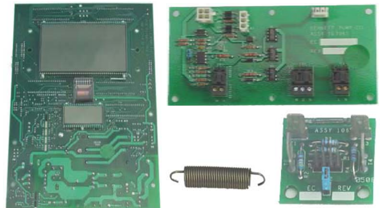
Electronics Package for a Master Big Squirt Hose CPU/Display ~ Satellite Board ~ Handle Switch Board ~ Handle Spring
